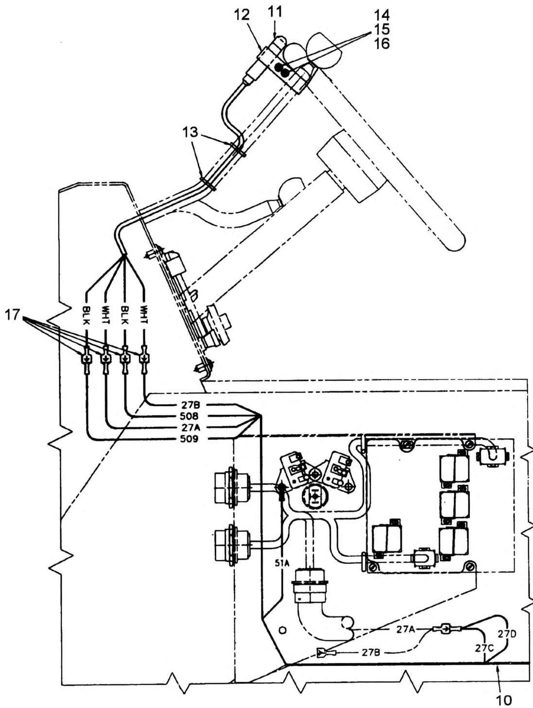
VIEW A - A
